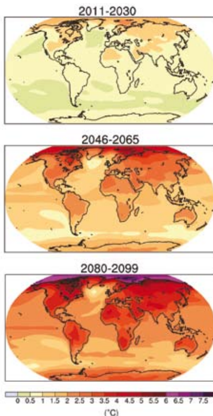
Map showing how the world will warm by the early, mid and late 21st century for a medium-high emissions scenario.
